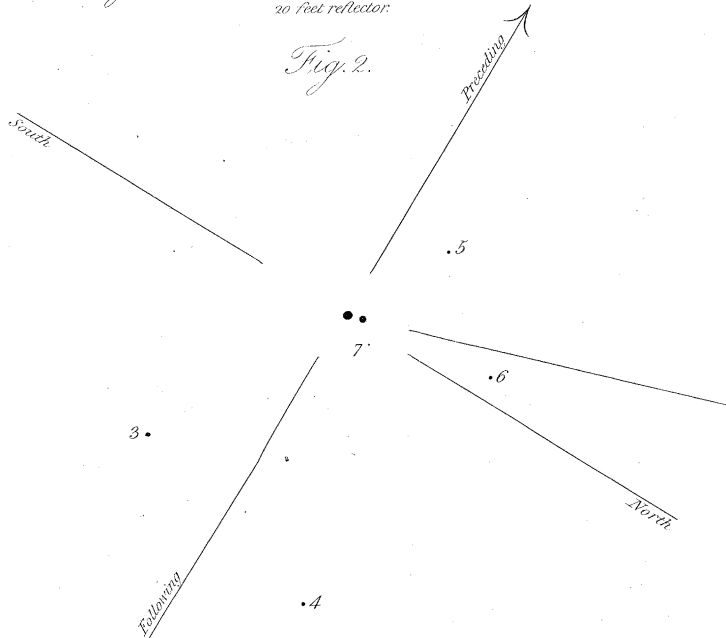
Fig. 2. \xi Bootis and the neighbouring Stars. 20 feet reflector.
