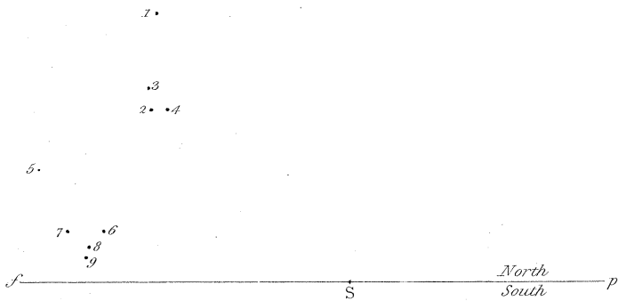
Fig. 4. Shewing the different relative positions of the two Stars 61 Cygni and its companion at different times and according to different observers.
