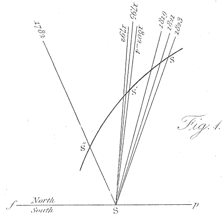
Fig. 1. The apparent relative orbit of the two Stars of \xi Bootis.
