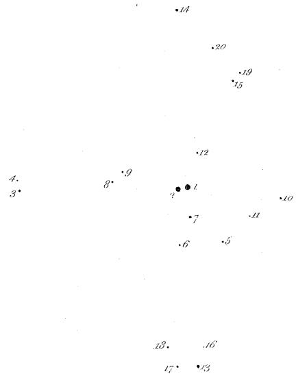
Fig. 3; 61. Cygni and the neighbouring Stars. as seen in the 20 feet reflector Sep. 16. 1823.
