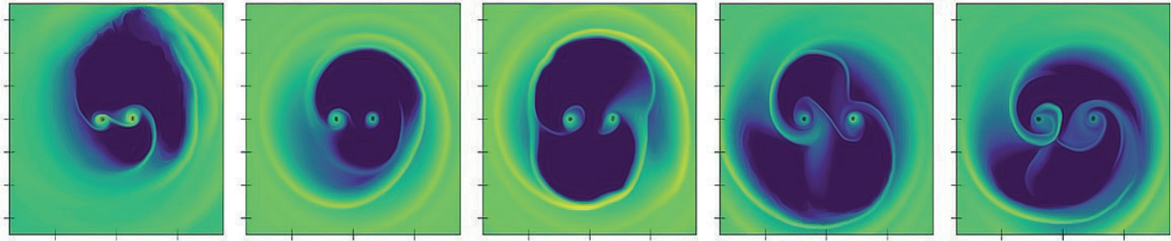
Fig 1. Snapshots of the hydrodynamical simulations produced by Siwek and collaborators.
