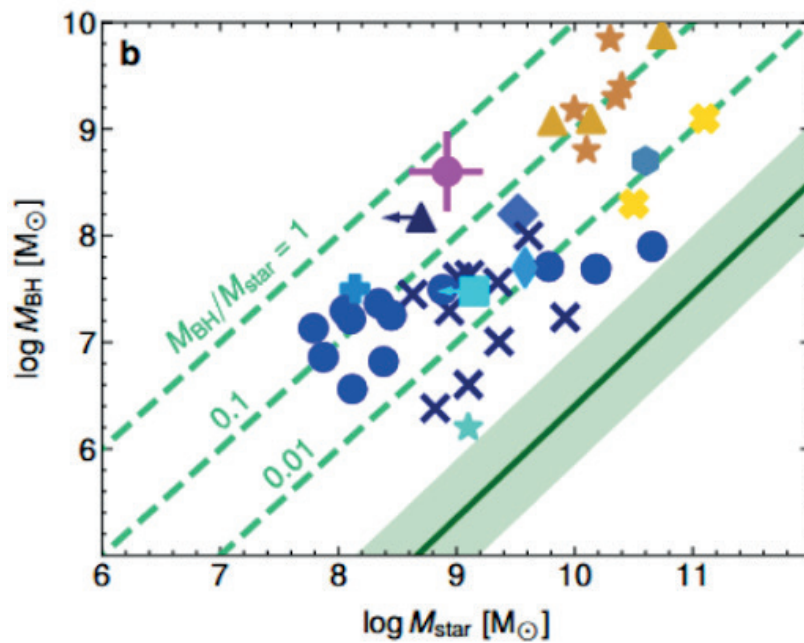
Fig 2. A galaxy with a 'dormant' black hole discovered by JADES, enabling an accurate measurement of both the mass of the black hole and the galaxy's stellar mass (magenta circle with error bars). This system has been crucial for confirming the existence of galaxies with 'over-massive' black holes, i.e., with high black hole-to-stellar mass ratio compared to the local scaling relation (solid green line). Figure from Juodžbalis et al. (2024a).
