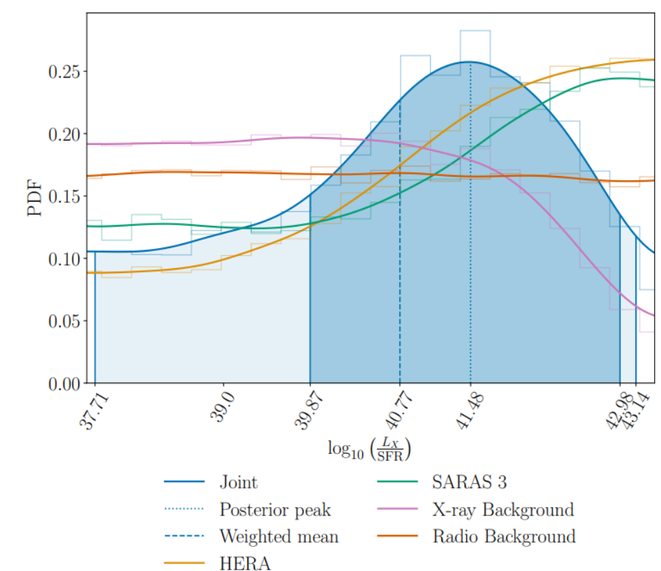
Fig 1. Probability density for the X-ray efficiency parameter. The peak appears due to the X-ray data (magenta) and 21-cm data (HERA in orange and SARAS 3 in green) weakly constraining opposite ends of the parameter range. The X-ray efficiency is unconstrained by radio background data (red). The joint fit (blue) reveals a distinct posterior peak (dotted vertical line) in the log X-ray luminosity per star formation rate of high-redshift X-ray binaries.
