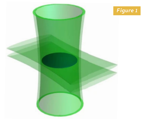
Fig 1. The planned experiment uses a “box trap” made of laser light to confine ultra-cold atoms into a 2D plane. Image from Navon N. et al., Nat. Phys. 17, 1334–1341 (2021).
